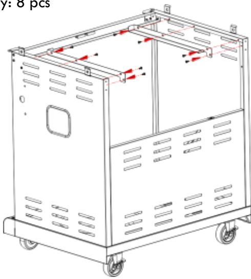
M4x10 Screw Qty: 8 pcs
