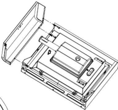
M6x13 Screw Qty: 3 pcs
