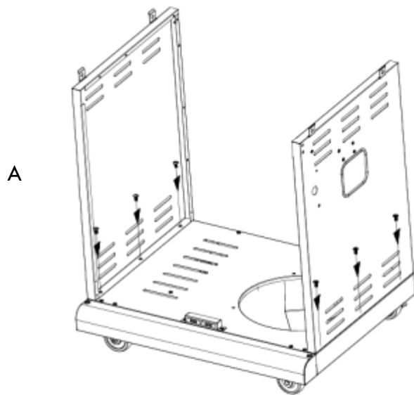
M6x13 Screw Qty: 6 pcs
